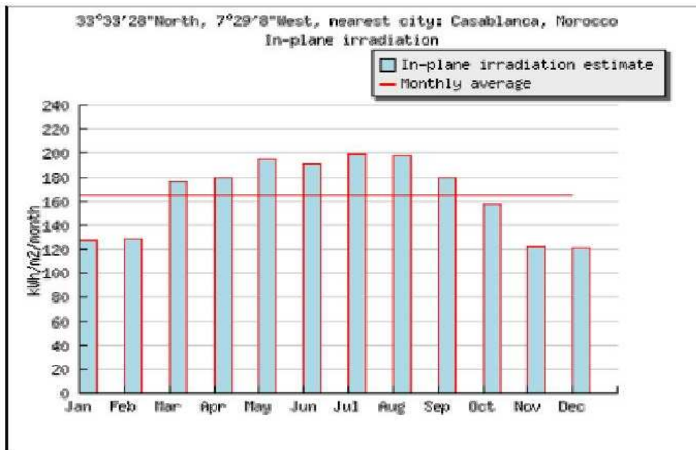
Figure 4.4: In-plane global irradiation estimated for the optimal inclination and orientation of Chourouk PV modules. The estimated monthly average value is also shown.
